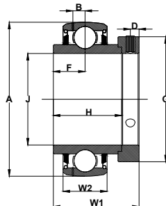
Type 2 Spherical outer ring - Inner ring extended both sides.
